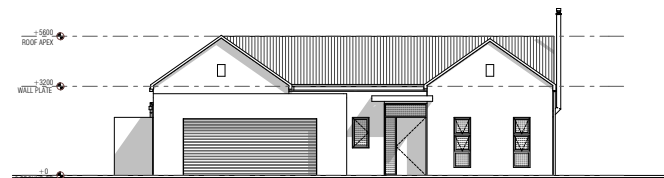
SOUTH ELEVATION 1:100
