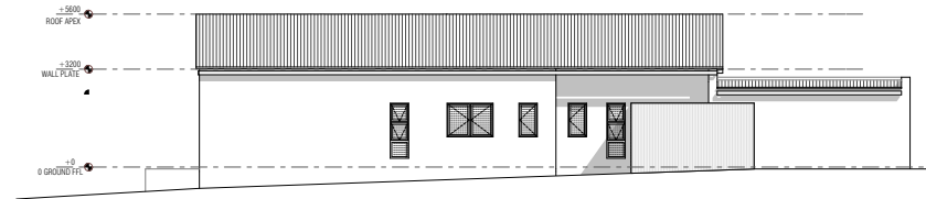
WEST ELEVATION 1:100
