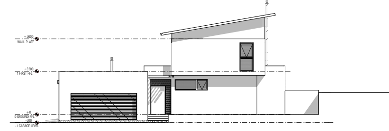
WEST ELEVATION 1:100
