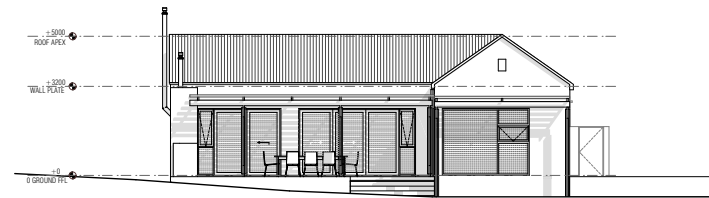
WEST ELEVATION 1:100
