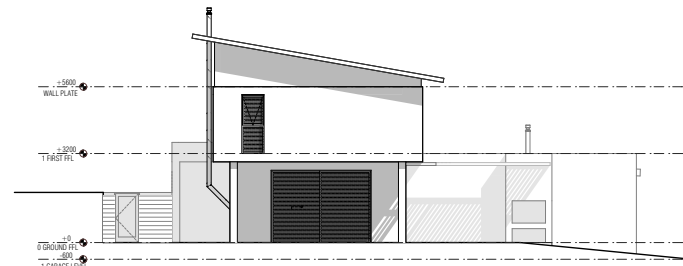
EAST ELEVATION 1:100
