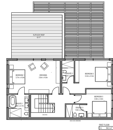
FIRST FLOOR 1:100
